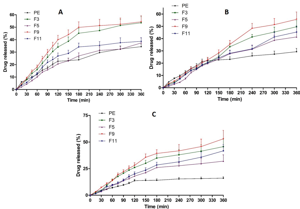
Figure 5. In vitro dissolution profiles of CA (A), QU (B) and KP (C) in PE in comparison with different PEP formulations in FaSSGF, pH 1.6 at 37 °C (means \pm SD, n = 3 ).
