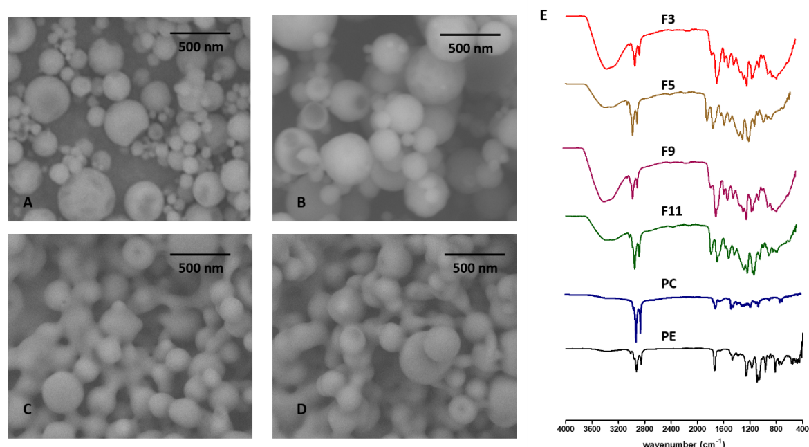
Figure 4. SEM images of F3 (A), F5 (B), F9 (C) and F11 (D) formulation of PEP at a magnification power of 30000x. FTIR spectra of F3, F5, F9 and F11 formulation of PEP, PC and PE (E).
