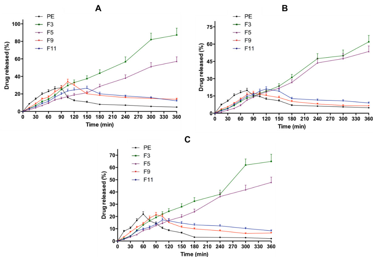
Figure 6. In vitro dissolution profiles of CA (A), QU (B) and KP (C) in PE in comparison with different PEP formulations in FeSSIF, pH 5.0 at 37 °C (means \pm SD, n = 3 ).
