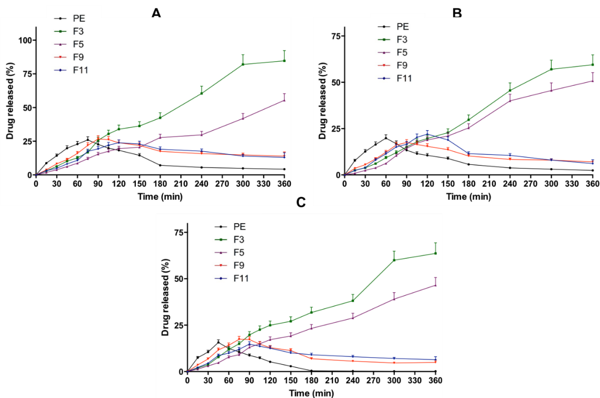
Figure 7. In vitro dissolution profiles of CA (A), QU (B) and KP (C) in PE in comparison with different PEP formulations in FaSSIF, pH 6.5 at 37 °C (means \pm SD, n = 3 ).
